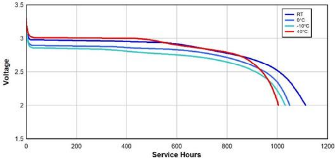
Temperature Discharge 30K Ohm Continuous to 2.0V
